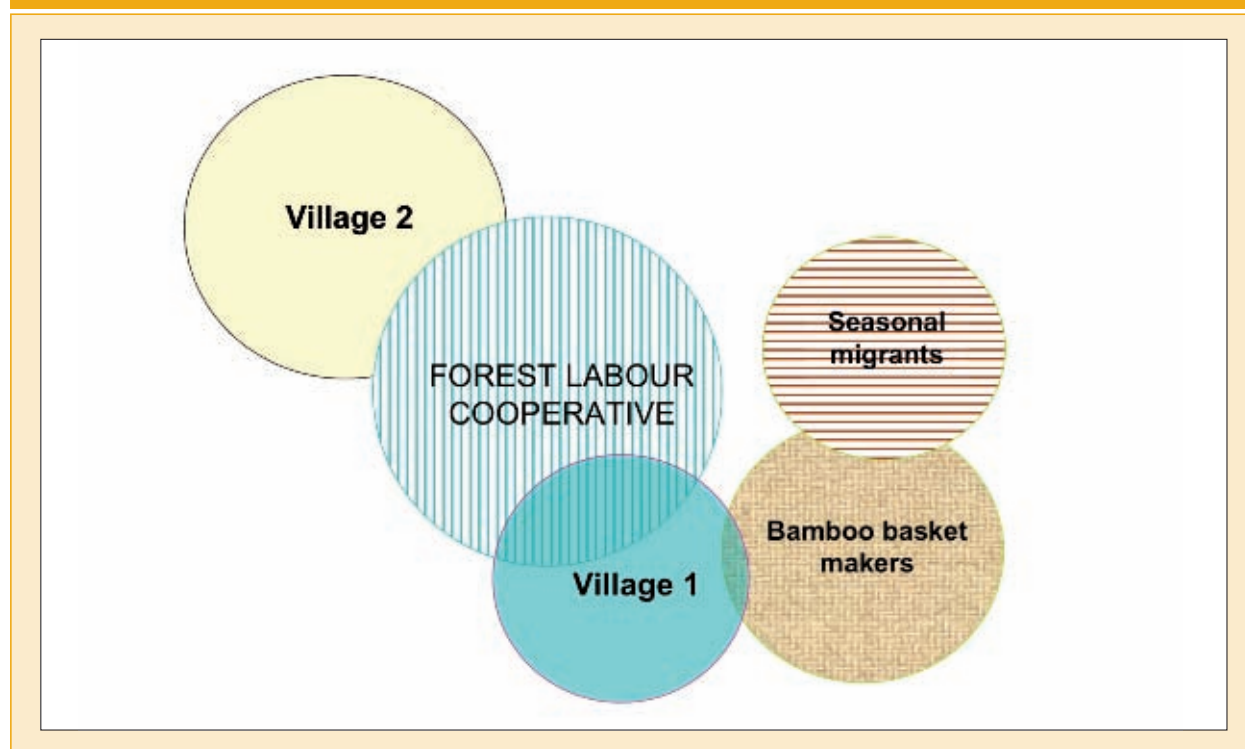
Figure 3.2 Venn diagram
